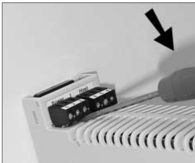
Figure 10 - Disconnection of FNICO power supply terminal block
