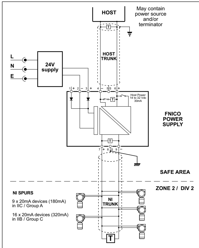
Figure 2 - Block diagram of simple FNICO system
