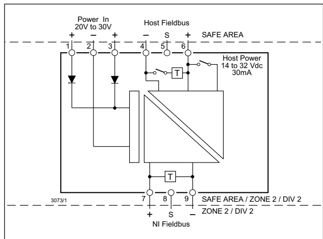
Figure 14 - Field location of FNICO power supply
