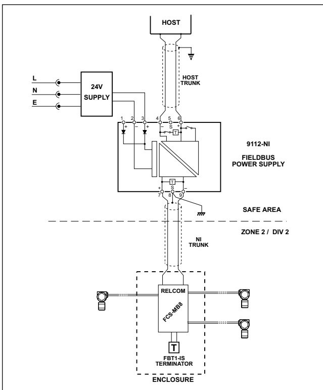
Figure 26 - Typical installation
